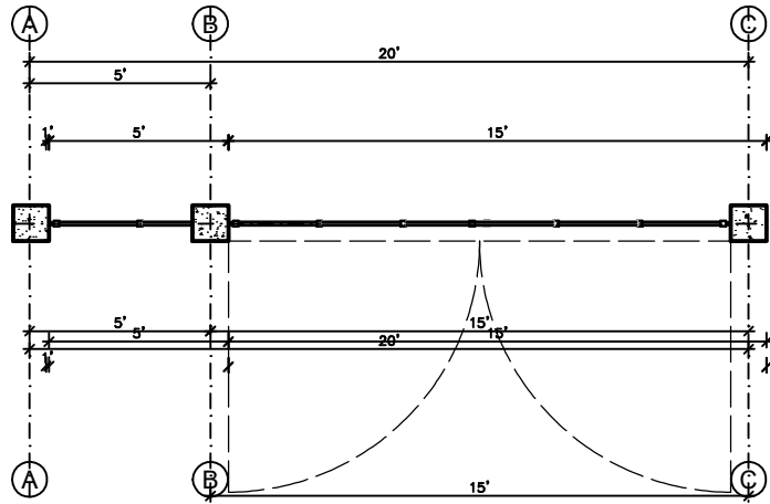
MAIN ENTRANCE GATE PLAN
