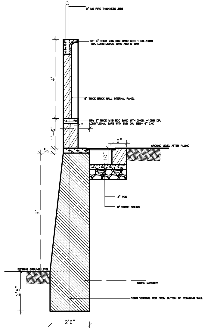
SECTION 4-4
