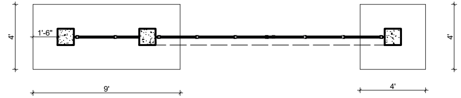
TRENCH PLAN FOR GATE COLUMN
