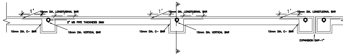
PLAN VIEW:- TOP BAND REINFORCEMENT DETAILING
