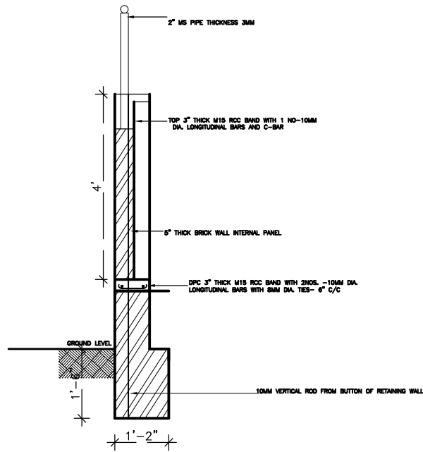
SECTION 1-1
