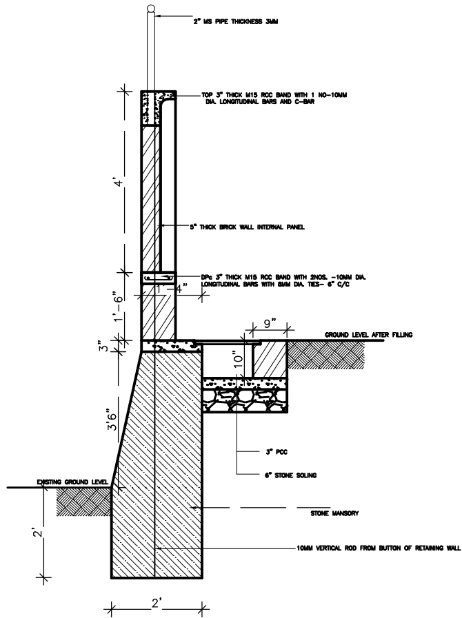
SECTION 3-3
