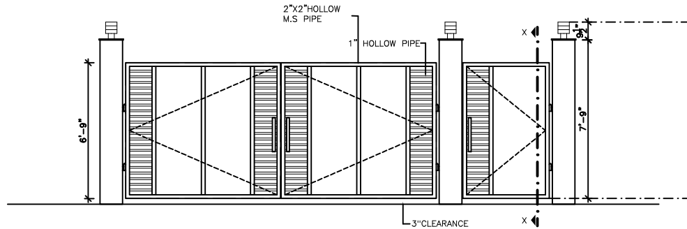
MAIN ENTRANCE GATE FRONT ELEVATION
