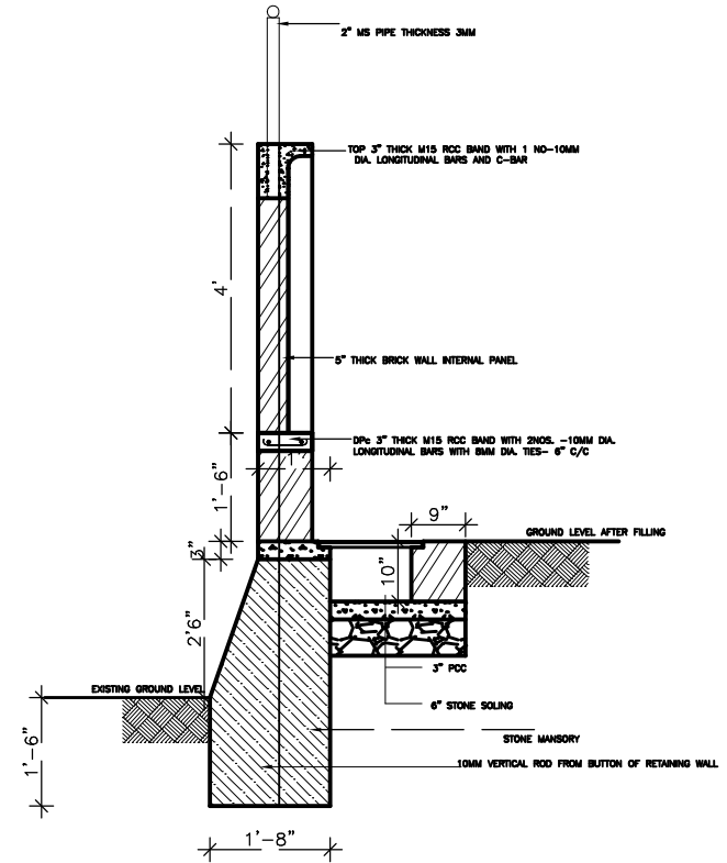
SECTION 2-2
