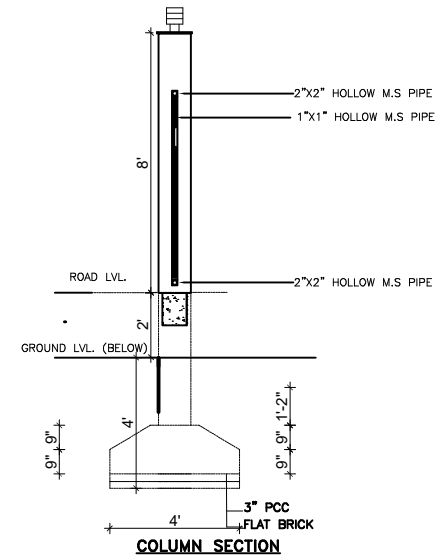
COLUMN SECTION
