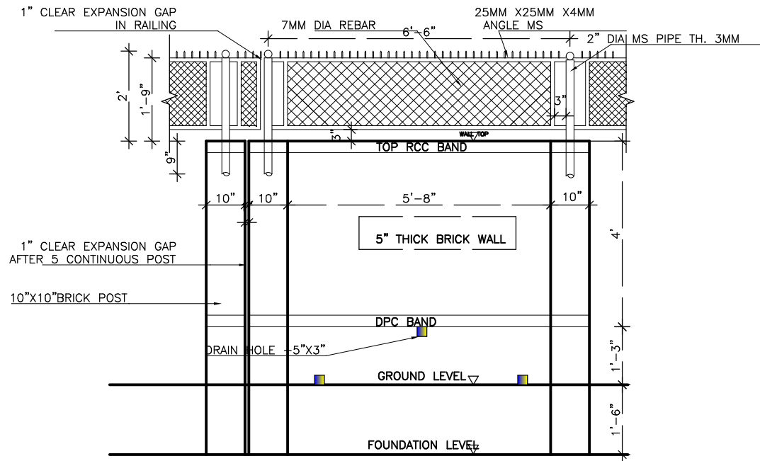
BOUNDARY WALL DETAILS
